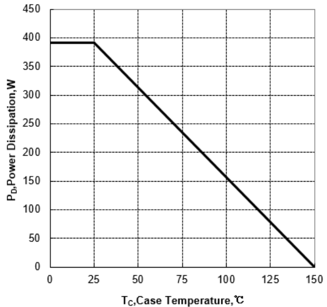
Figure 2 Power Dissipation
