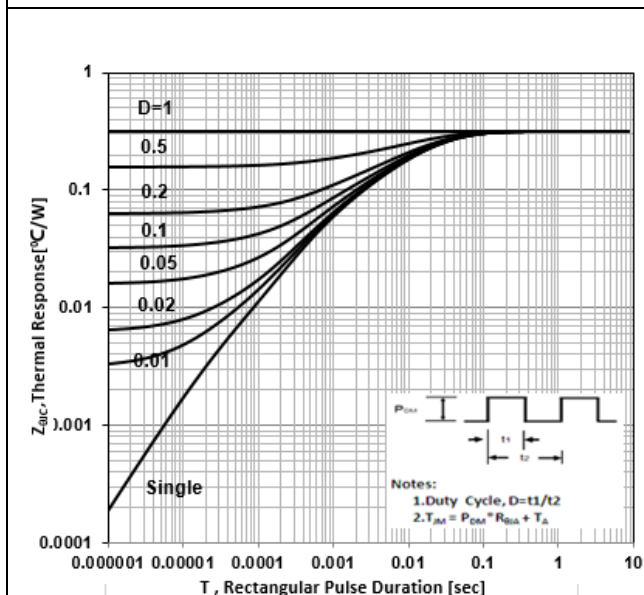
Figure 3 Max Thermal Impedance
